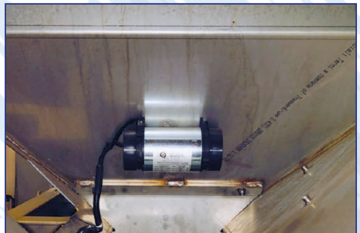
Electric vibrator 12 V 24 V to ease the salt removal from the internal part of the hopper
